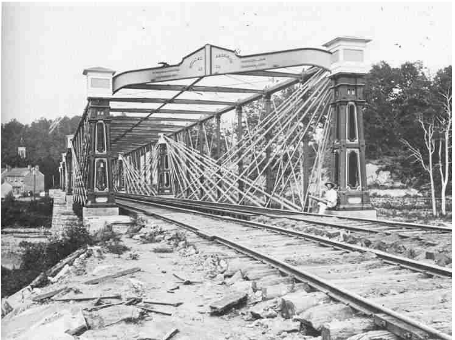
BOLLMAN TRUSS, B & O, ALBERTON, MARYLAND (story inside)
